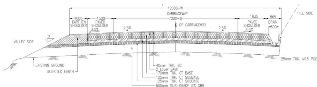
TYPICAL PAVEMENT DETAILS FOR MAIN ROAD
